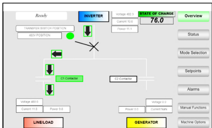
Generator Idle
