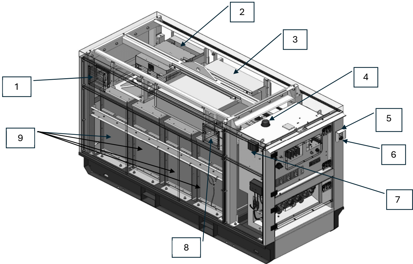
Component List – Isometric View
