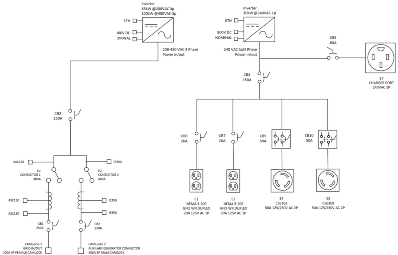
Single Line Electrical System Diagram
